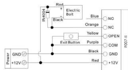
Common Power Supply Connection Diagram
